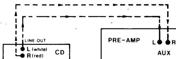
Figure 4 External Connections
